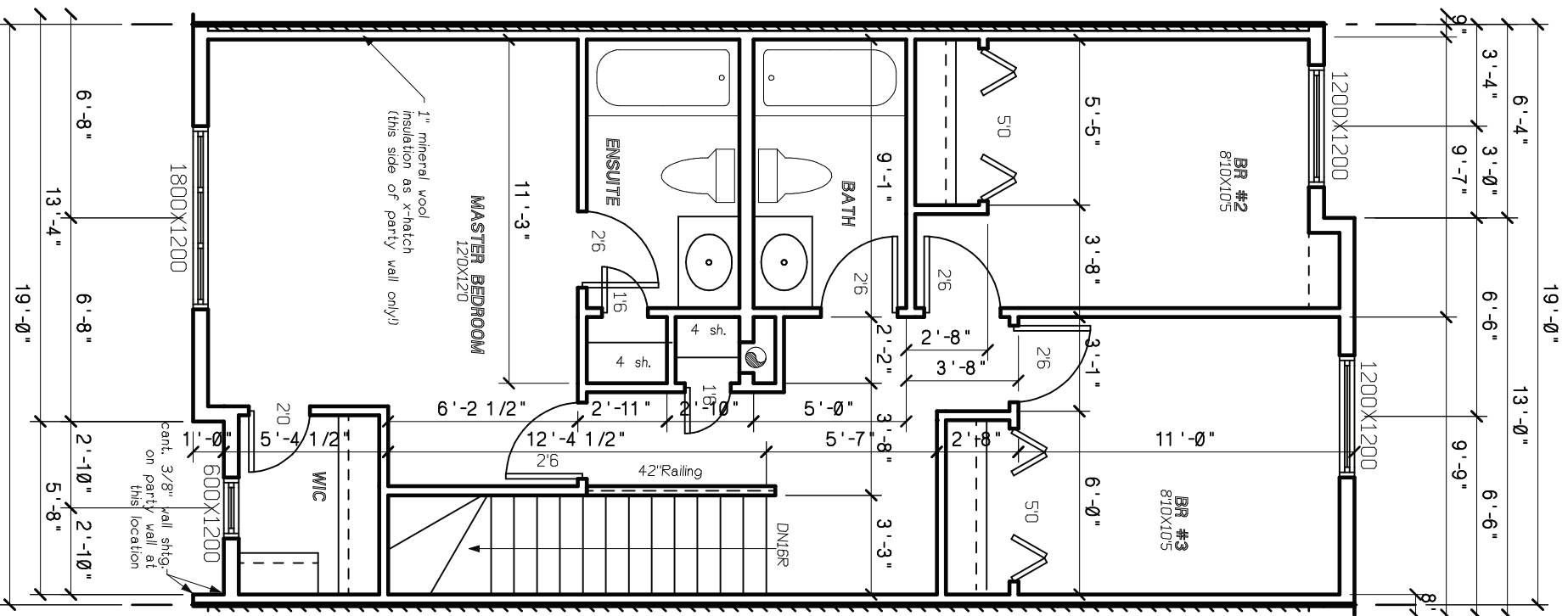
SECOND FLOOR - 708sq.ft. 3C
